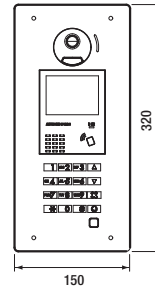
Flush mount with GF-3B
